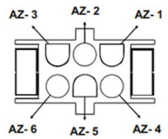
CONECTOR HYLOCK
